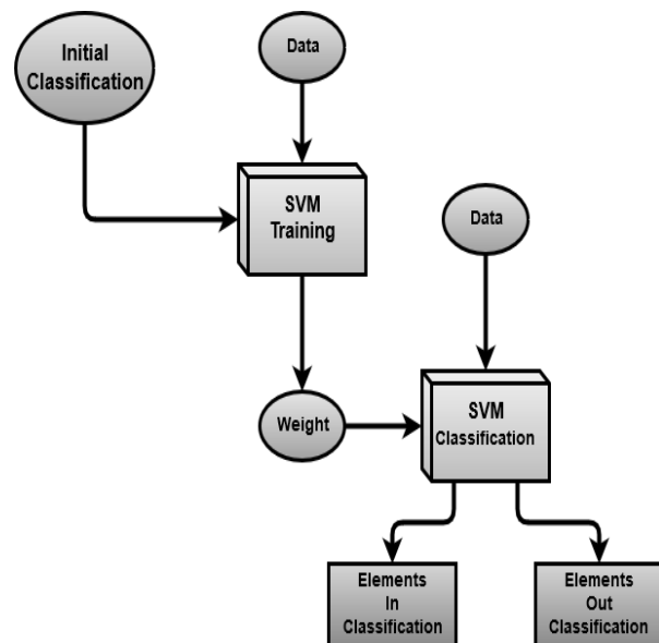
Fig.1 Support Vector Machine Model Execution
