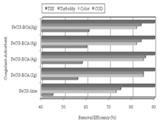
Fig.5: Treatment of industrial dyes wastewater using \text{FeCl}_3 -Lime and BBCA adsorbent at dose variations.
