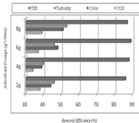
Fig.4: Treatment of industrial dyes wastewater through bottom based Coal ash with variant doses.
