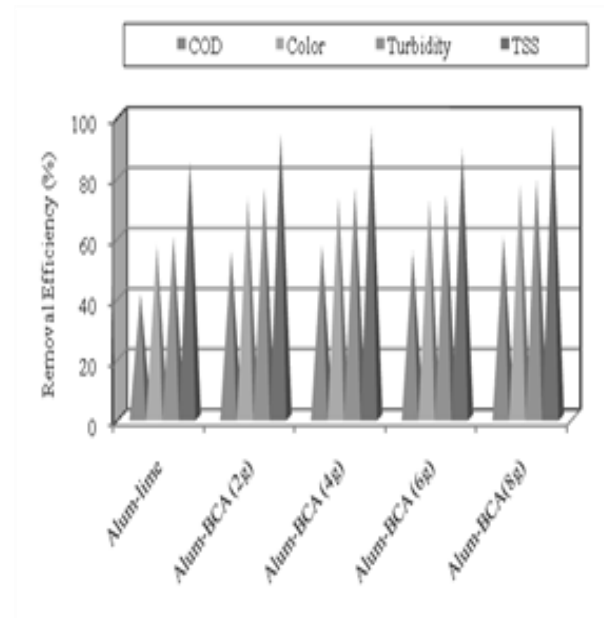
Fig.7: Treatment of industrial dyes wastewater using Alum-lime and BCCA- adsorbent at dose variations.
