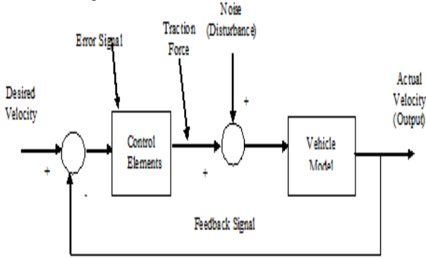
Fig. 3. Block diagram for the feedback control system.
